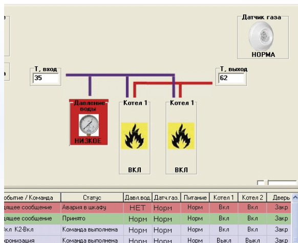
System heat supply dispatching control
