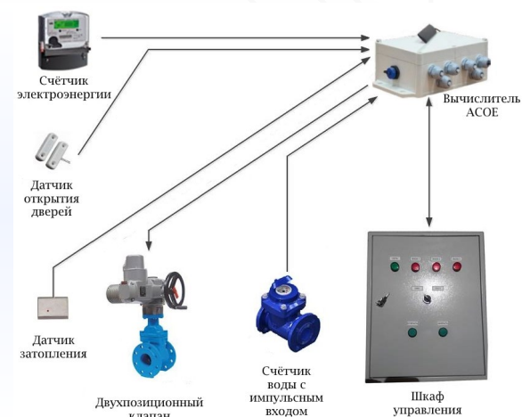
Dispatching system of pumping stations
