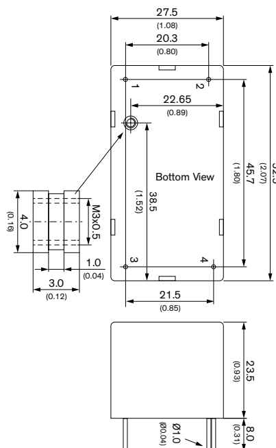
Pin Connections
