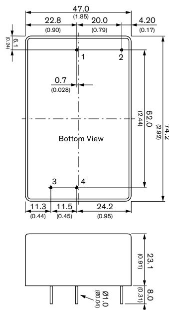
Pin Connections
