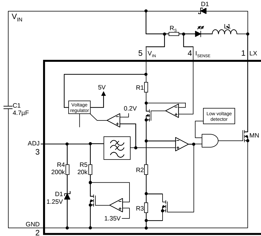
Figure 1. Block diagram – With Pin Connections
