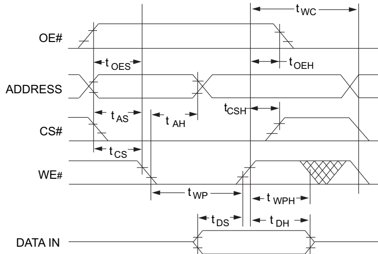
FIGURE 4 – WRITE WAVEFORMS WE# CONTROLLED
