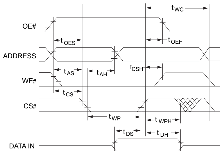
FIGURE 5 – WRITE WAVEFORMS CS# CONTROLLED
