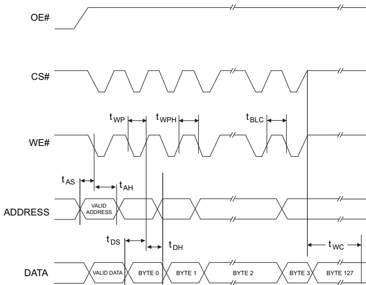
FIGURE 7 – PAGE MODE WRITE WAVEFORMS
