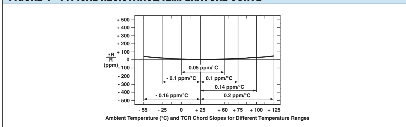
FIGURE 4 - TYPICAL RESISTANCE/TEMPERATURE CURVE
