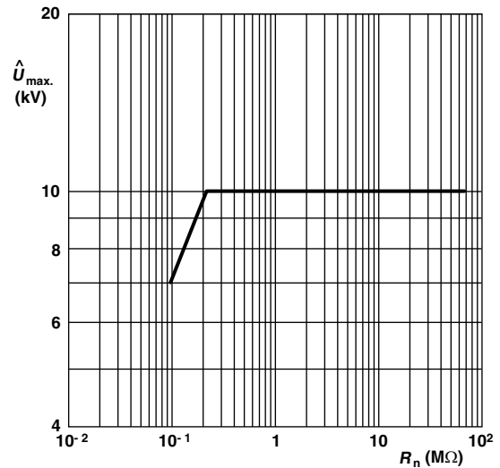
Maximum allowed peak pulse voltage in accordance with IEC 60065, 14.1.a) *) ; 50 discharges from a 1 nF capacitor charged to \hat{U}_{max.} ; 12 discharges/minute (drift \Delta R/R \leq 2\% )
