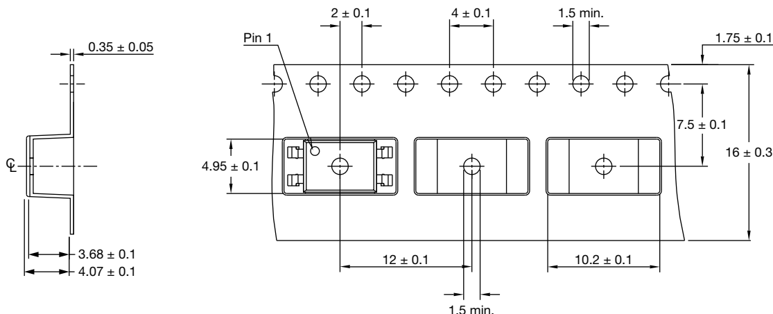
Fig. 16 - Tape and Reel Packing
