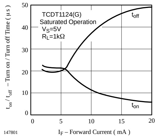
Figure 18. Turn on / off Time vs. Forward Current
