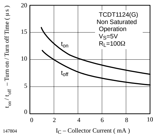
Figure 21. Turn on / off Time vs. Collector Current
