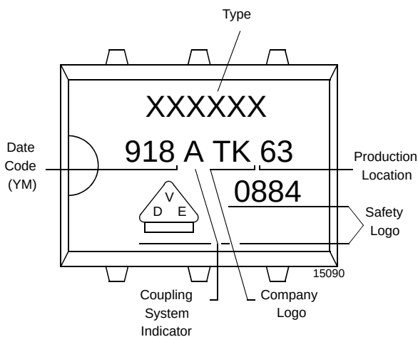
Figure 22. Marking example
