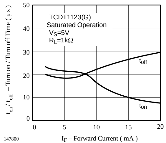
Figure 17. Turn on / off Time vs. Forward Current
