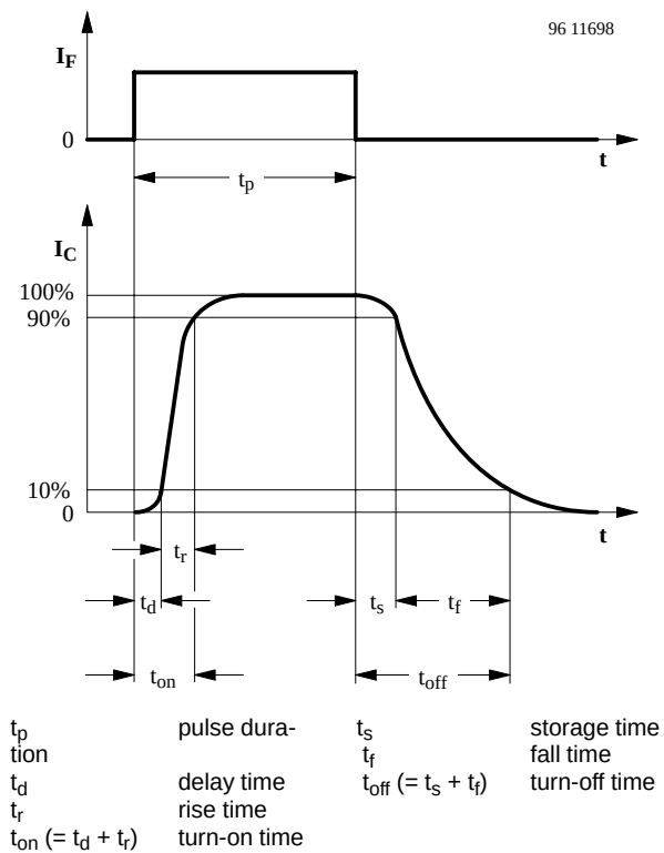
Figure 5. Switching times
