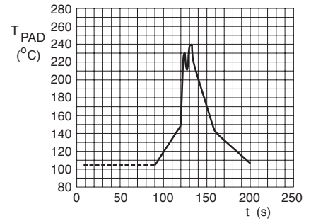
Fig. 6 Maximum temperature load during (double-) wave soldering.
