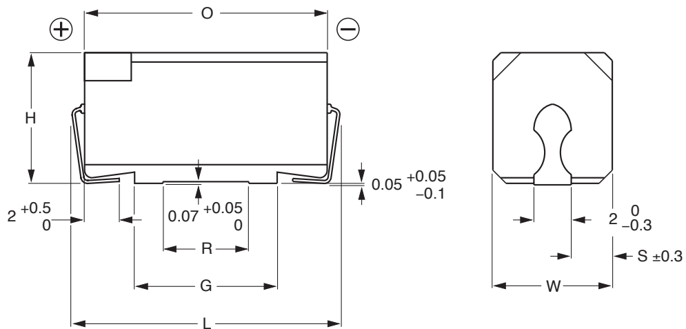
Fig.2 Dimensional outline.
