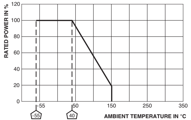
Derating KKE.. Si
