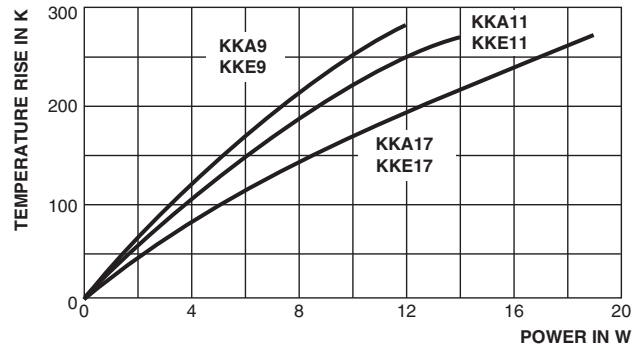
Temperature Rise
