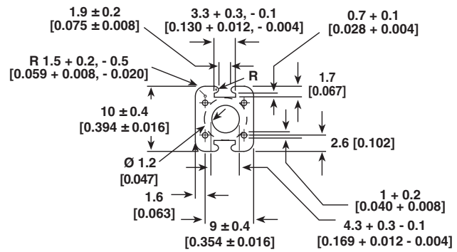
Profile dimensions
