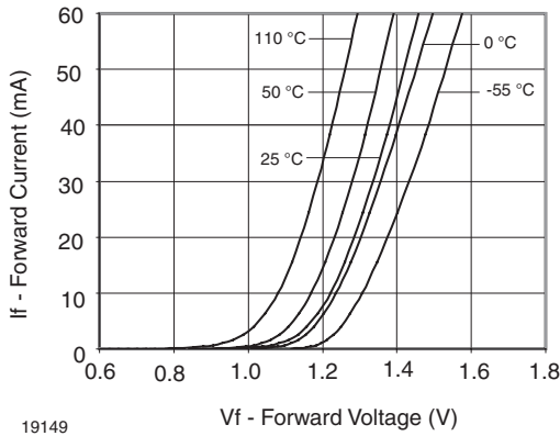
Figure 3. Forward Current vs. Forward Voltage
