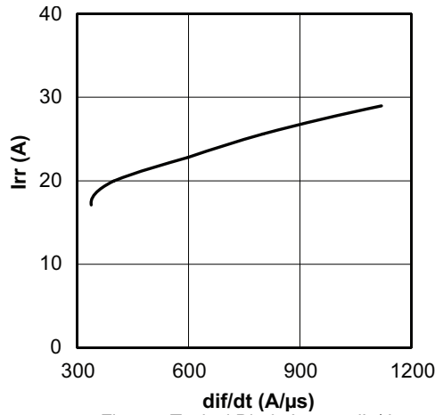
Fig. 34 - Typical Diode I_{RR} vs. \text{di}/\text{dt} V_{CC} = 300\text{ V} ; V_{GE} = 15\text{ V} ; I_{CE} = 10\text{ A} ; T_J = 125^\circ\text{C}
