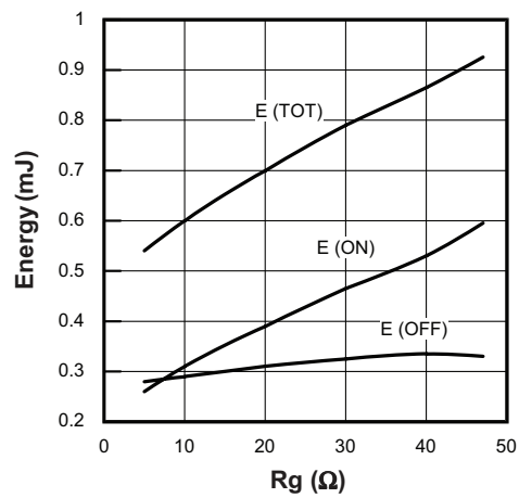
Fig. 11 - Typical Energy Loss vs. R_G T_J = 125\text{ }^\circ\text{C} ; L = 200\text{ }\mu\text{H} ; V_{CE} = 300\text{ V} ; I_{CE} = 20\text{ A} ; V_{GE} = 15\text{ V}
