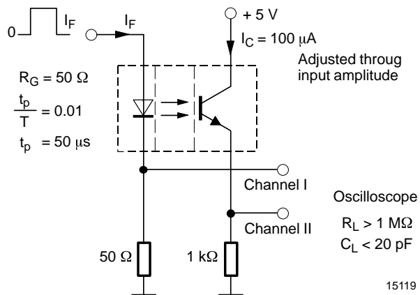
Figure 1. Test circuit
