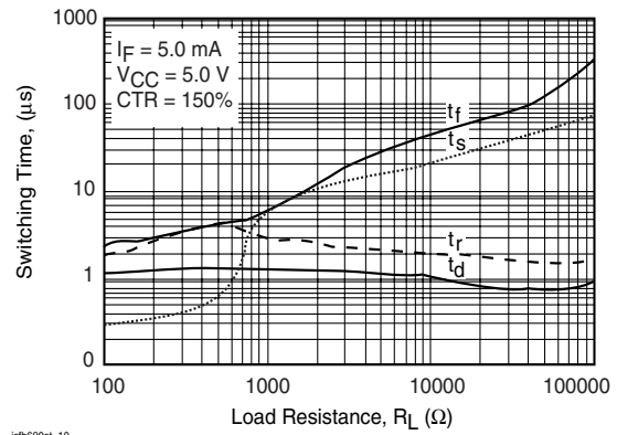
Figure 11. Switching Time vs. Load Resistance
