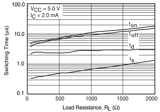
Figure 10. Switching Time vs. Load Resistance
