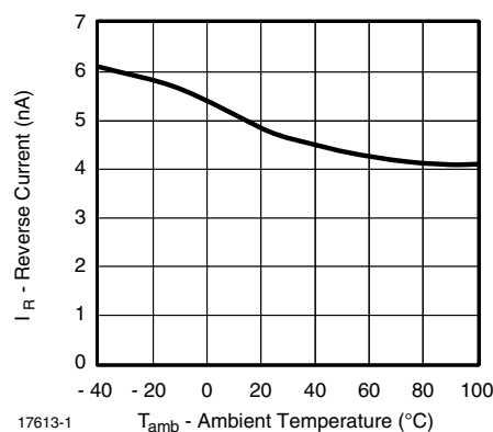
Figure 5. Reverse Current vs. Ambient Temperature
