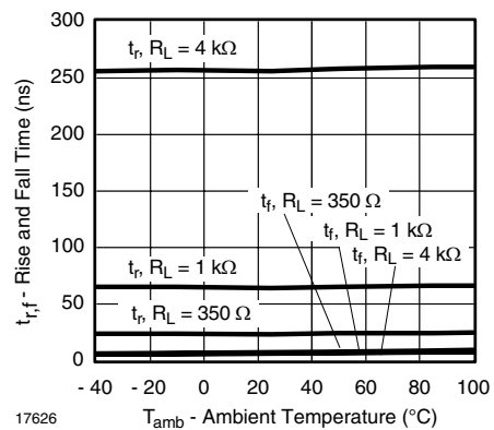
Figure 18. Rise and Fall Time vs. Ambient Temperature
