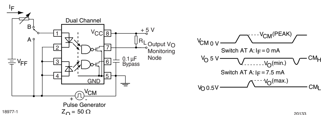
Figure 2. Dual Channel Test Circuit for Common Mode Transient Immunity
