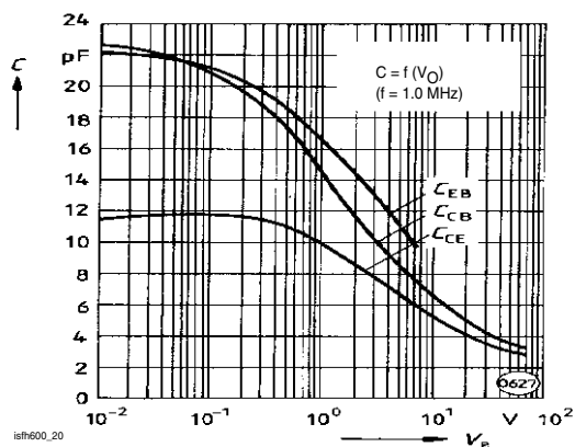
Figure 20. Transistor Capacitance
