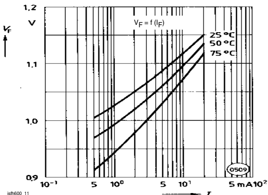
Figure 11. Forward Voltage
