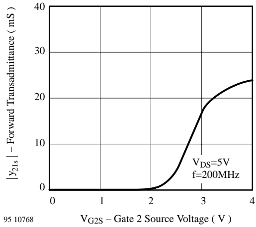
Figure 4. Forward Transmittance vs. Gate 2 Source Voltage
