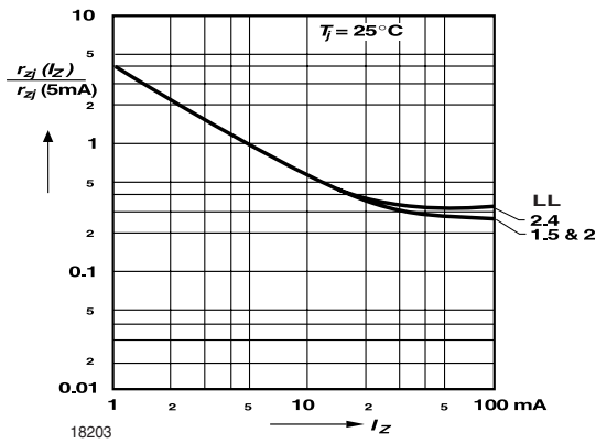
Figure 4. Dynamic resistance vs. operating current, normalized
