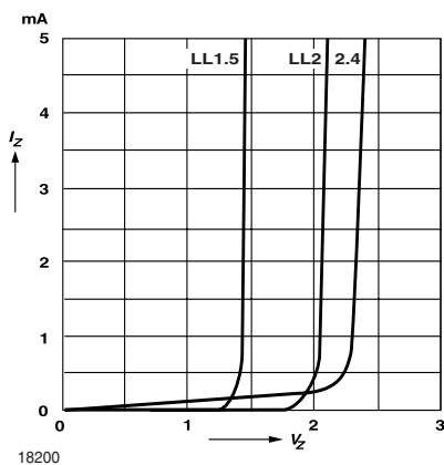
Figure 1. Breakdown Characteristics
