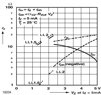
Figure 5. Dynamic resistance vs. operating voltage
