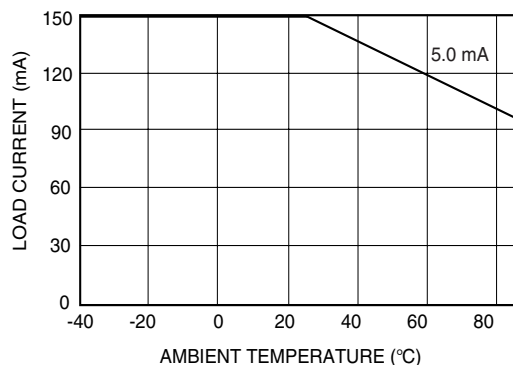
Figure 1. Recommended Operating Conditions
