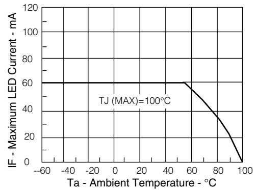
Figure 7. Maximum LED current versus ambient temperature
