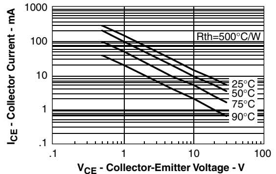
Figure 15. Maximum collector current versus collector voltage
