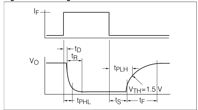
Figure 8. Switching waveforms
