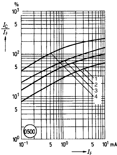
Figure 3. Current transfer ratio versus diode current ( T_A=-25^\circ\text{C} , V_{CE}=5.0\text{ V} ) I_C/I_F=f(I_F)
