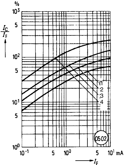
Figure 4. Current transfer ratio versus diode current ( T_A=0^\circ\text{C} , V_{CE}=5.0\text{ V} ) I_C/I_F=f(I_F)
