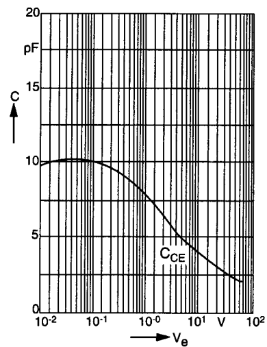
Figure 19. Transistor capacitance C=f(V_O) ( T_A=25^\circ\text{C} , f=1.0\text{ MHz} )
