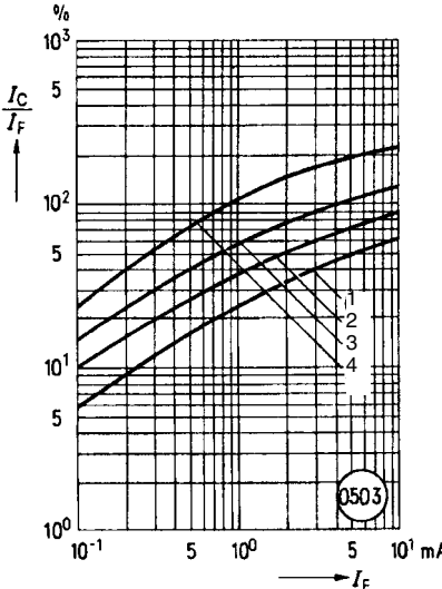
Figure 5. Current transfer ratio versus diode current ( T_A=25^\circ\text{C} , V_{CE}=5.0\text{ V} ) I_C/I_F=f(I_F)
