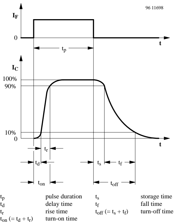
Figure 3. Switching times
