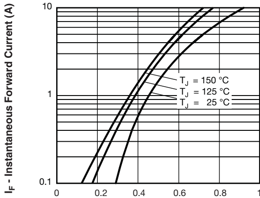
93320_01 V FM - Forward Voltage Drop (V) Fig. 1 - Maximum Forward Voltage Drop Characteristics
