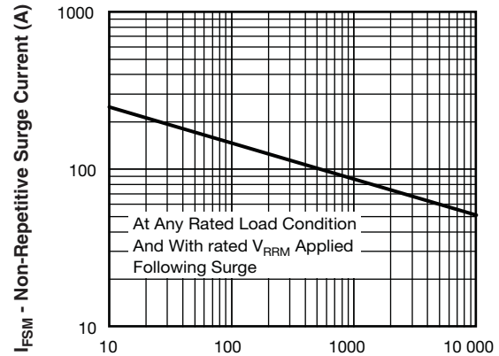
93320_06 t p - Square Wave Pulse Duration (μs) Fig. 6 - Maximum Non-Repetitive Surge Current
