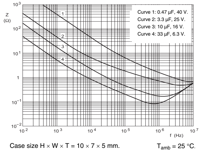
Fig.21 Typical impedance as a function of frequency.
