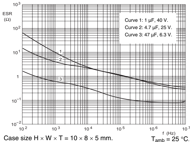
Fig.16 Typical ESR as a function of frequency.
