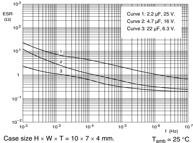
Fig.14 Typical ESR as a function of frequency.
