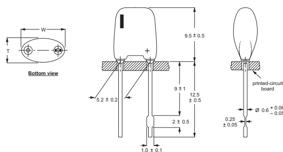
Fig.3 Form CA: Long leads with keyed polarity, in boxes.
