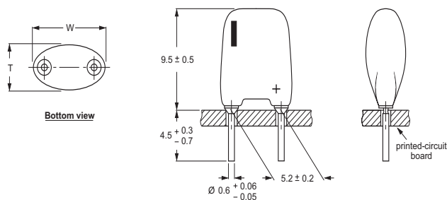
Fig.2 Form CB: Short leads, in boxes.
