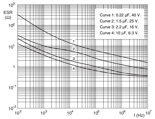
Case size H \times W \times T = 10 \times 7 \times 3.5 mm. T_{amb} = 25 °C. Fig.13 Typical ESR as a function of frequency.
