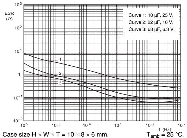
Fig.17 Typical ESR as a function of frequency.
