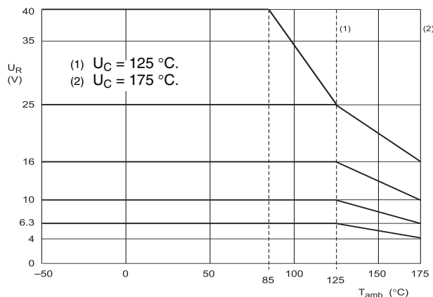
Fig.5 Maximum permissible voltage up to T_{amb} = 175^\circ\text{C} .
