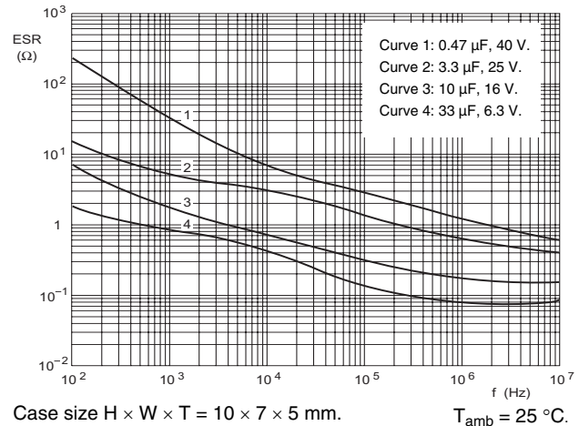
Fig.15 Typical ESR as a function of frequency.
