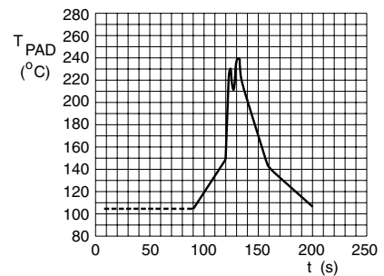
Fig.7 Maximum temperature load during (double-) wave soldering.
