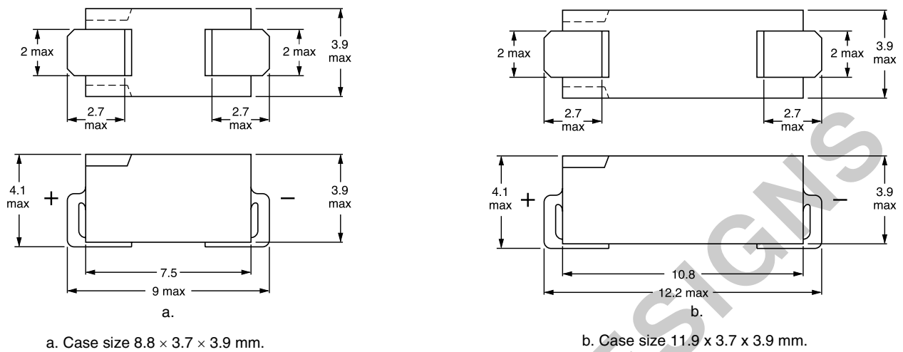
Fig.2 Dimensional outlines.
