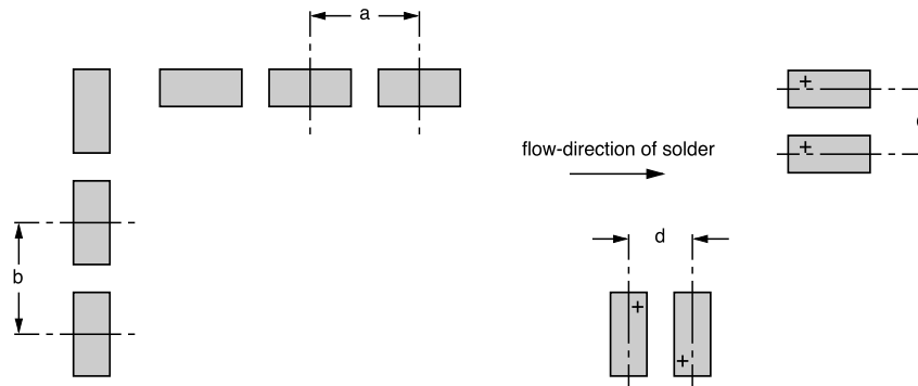
For dimensions a, b, c and d, refer to Table 3. Flow direction of solder preferably onto side-walls or plus-side of the capacitors.
