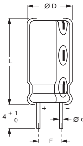
Fig.3 Form CB: Cut leads.
