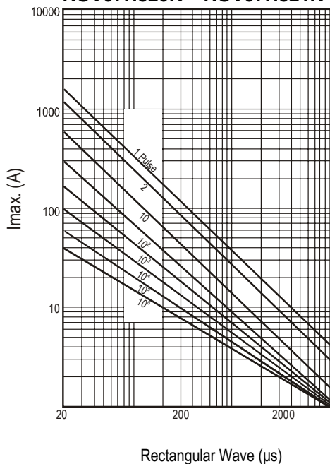
ROV07H820K – ROV07H821K
