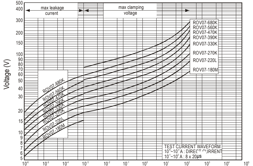
ROV07-180M – ROV07-680K
