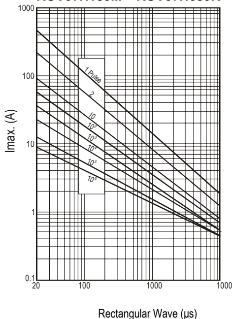
ROV07H180M – ROV07H680K
