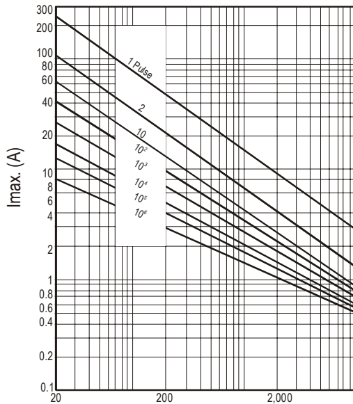
ROV07-180M – ROV07-680K
