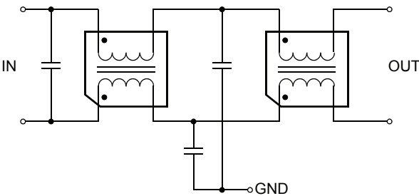
Figure 4. Internal Schematic
