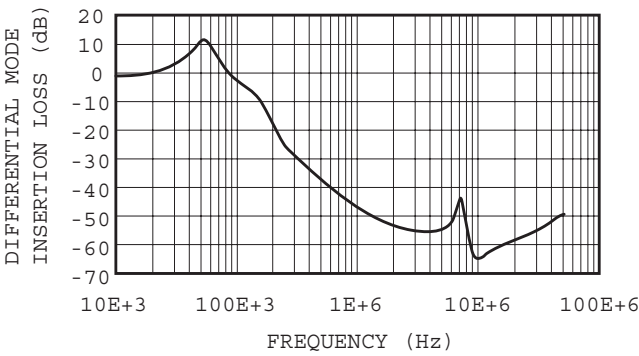
Figure 3. Typical Differential-Mode Insertion Loss in a 50 Ω Circuit
