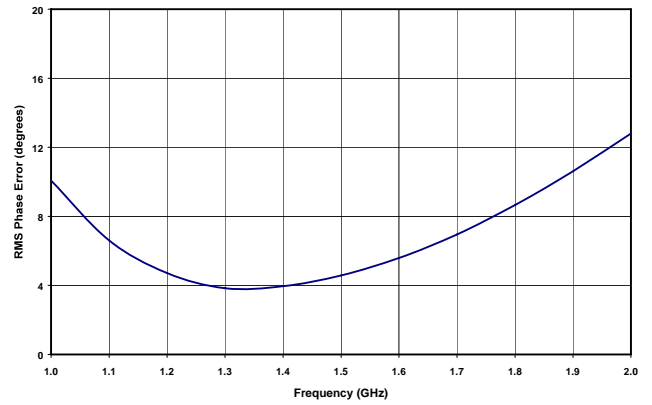
Figure 2. Corrected RMS Phase Error Over All Phase States
