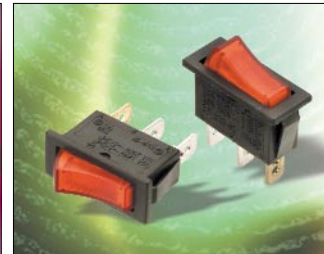
Series PRG 11.2 [.44] x 30.2 [1.19] Panel Cut-out
