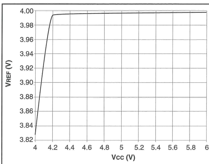
Figure 5. UCC3813-3/-5 V_{REF} vs. V_{CC} ; I_{LOAD} = 0.5mA .
