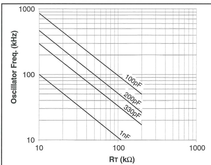
Figure 6. UCC3813-3/-5 oscillator frequency vs. R_T and C_T .
