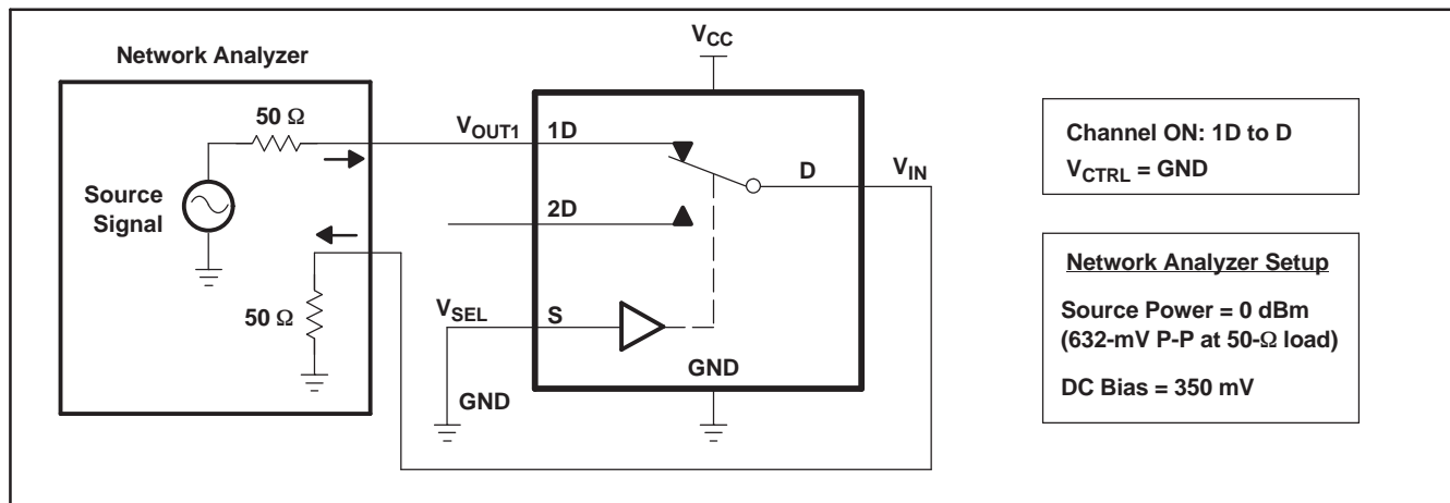
Figure 10. Bandwidth (BW)
