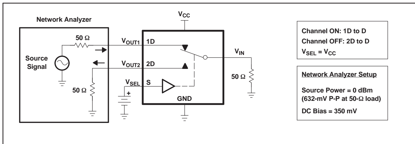
Figure 9. Crosstalk ( X_{TALK} )
