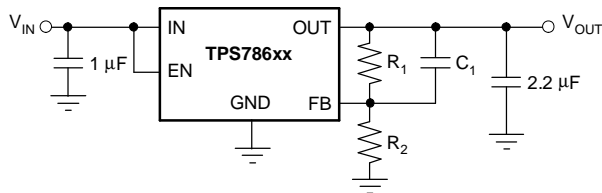
Figure 25. TPS78601 Adjustable LDO Regulator Programming
