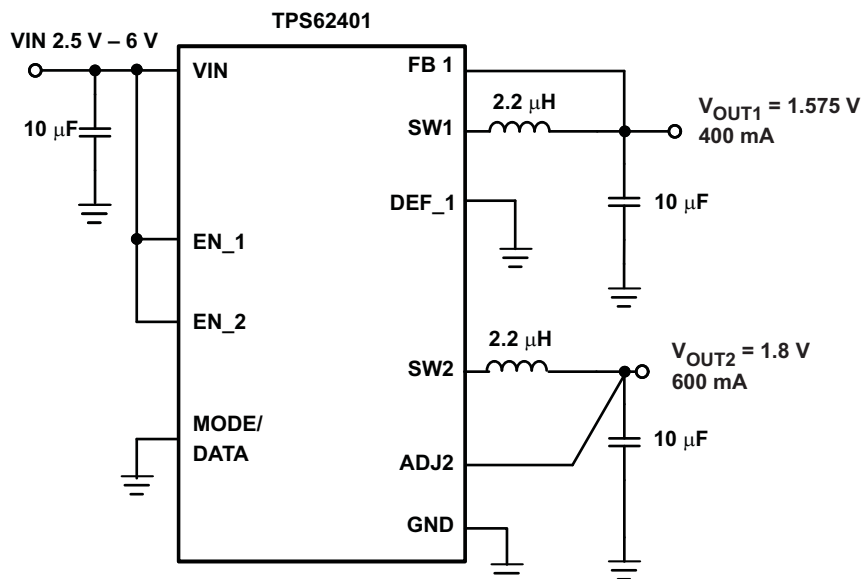
Figure 45. TPS62401 Fixed 1.575V/1.8V Outputs
