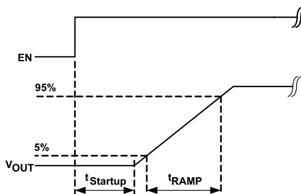
Figure 34. Soft Start
