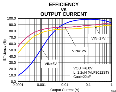
Figure 5. Vout=6V
