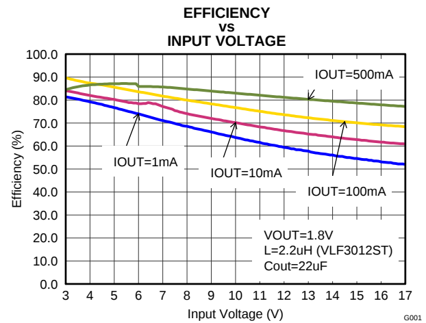
Figure 10. Vout=1.8V
