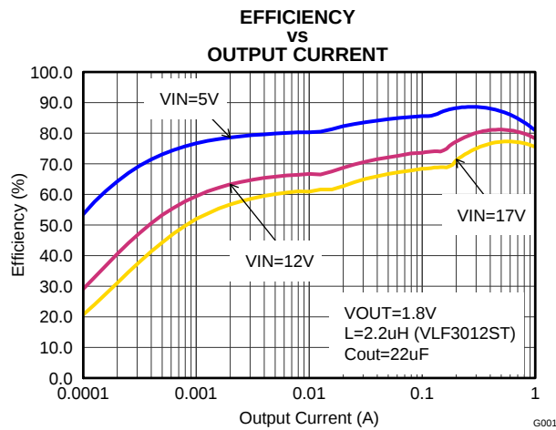
Figure 9. Vout=1.8V
