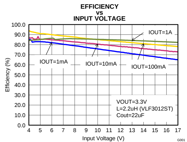
Figure 8. Vout=3.3V
