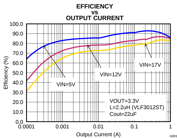
Figure 7. Vout=3.3V
