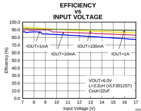
Figure 6. Vout=6V
