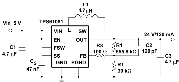
5 V to 24 V, 120 mA Step-up DC/DC Converter
