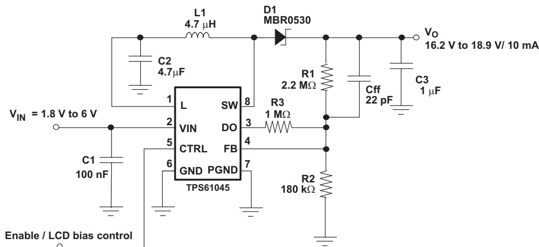
Figure 1. Typical Application
