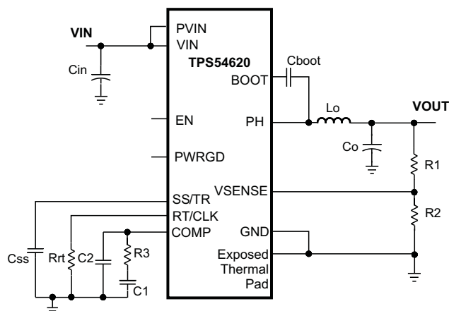
SIMPLIFIED SCHEMATIC
