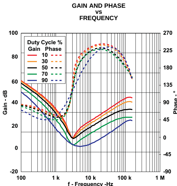
Figure 26. TPS54383 at 600-mApp Ripple Current
