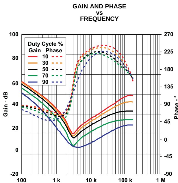
Figure 25. TPS54383 at 400-mA App Ripple Current
