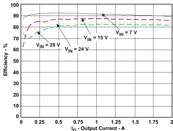
Figure 15. TPS54231 Efficiency
