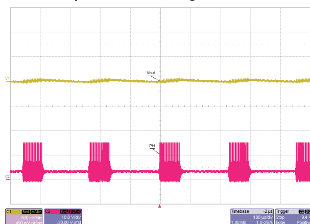
Figure 25. Eco-mode™
