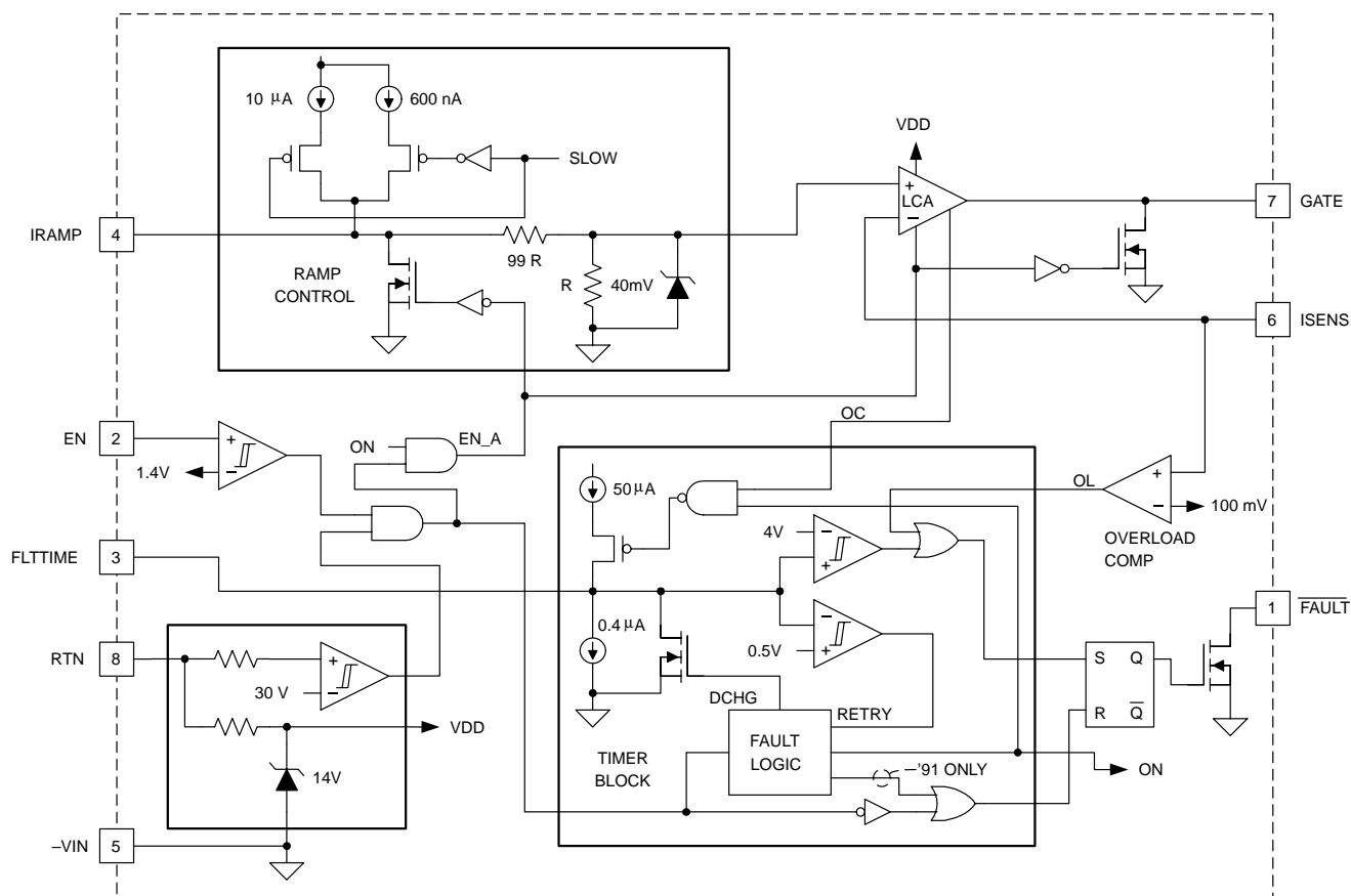
Figure 17. Block Diagram
