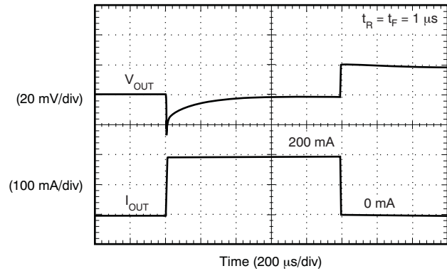
LOAD TRANSIENT 0
