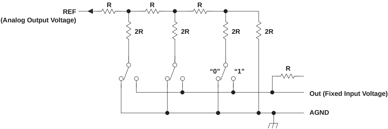
Figure 11. Voltage-Mode Operation
