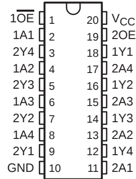
SN54HC241 . . . J OR W PACKAGE SN74HC241 . . . DW OR N PACKAGE (TOP VIEW)
