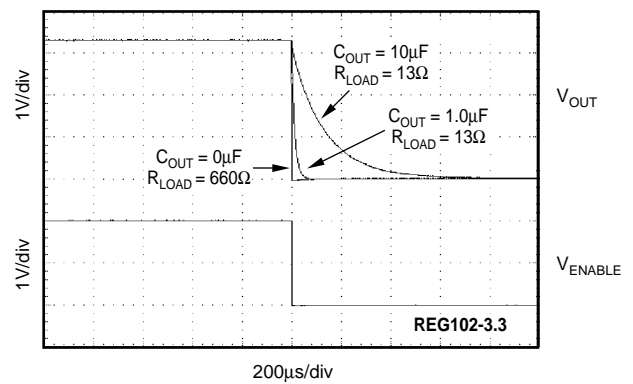
TURN-OFF
