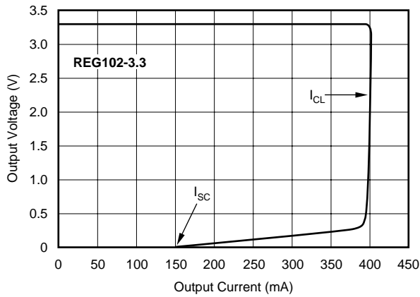
CURRENT LIMIT FOLDBACK
