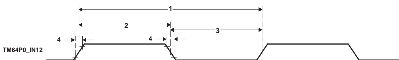
Figure 6-81. Timer Timing
