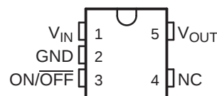
DBV (SOT-23) PACKAGE (TOP VIEW)
