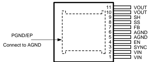
Figure 2. Top View 11-Lead PFM
