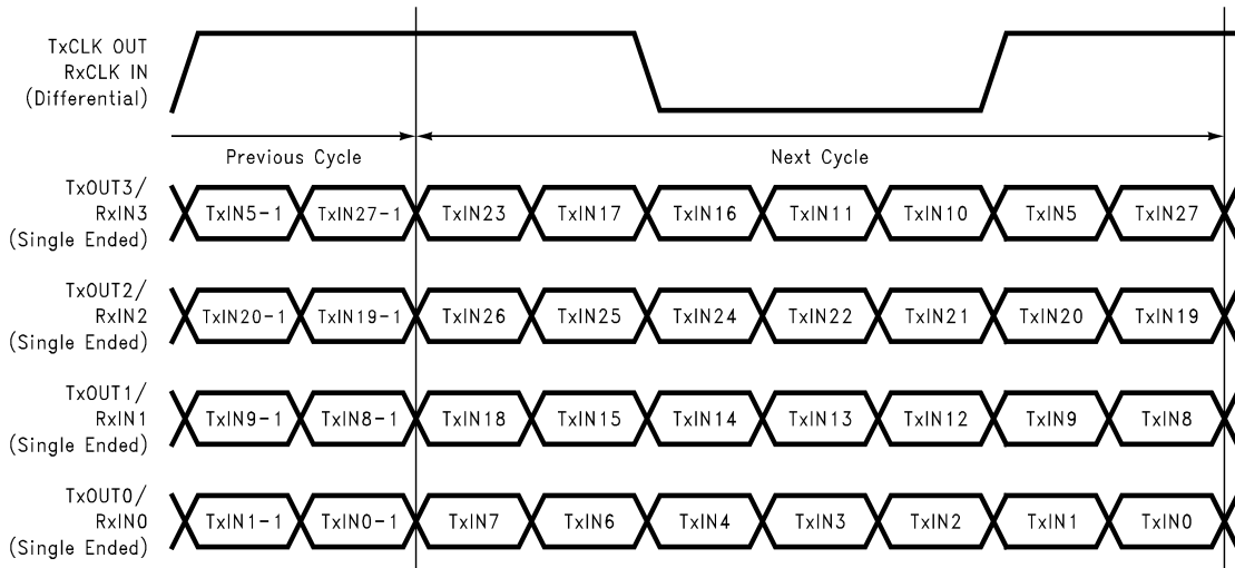
Figure 6. DS90CR286A Mapping of 28 LVC MOS Parallel Data to 4D + C LVDS Serialized Data
